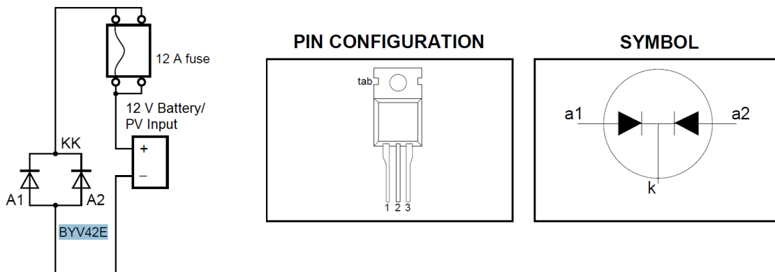
Figure 47 - BYV42E Rectifier Diode Connection, Configuration and Symbol. [60]
