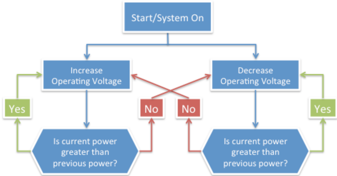
Figure 51 - Block Diagram of Perturb and Observe Method.
