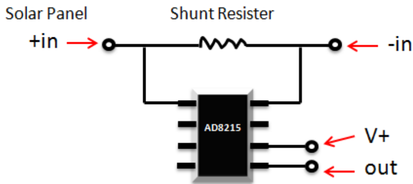
Figure 26 - AD8215 Current Shunt Monitor. [42]
