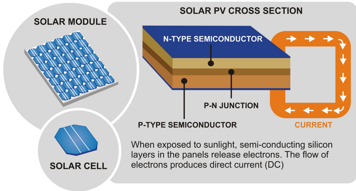
Figure 4 - Inside a Photovoltaic Cell. Permission requested from Ikhwezi Unplugged.
