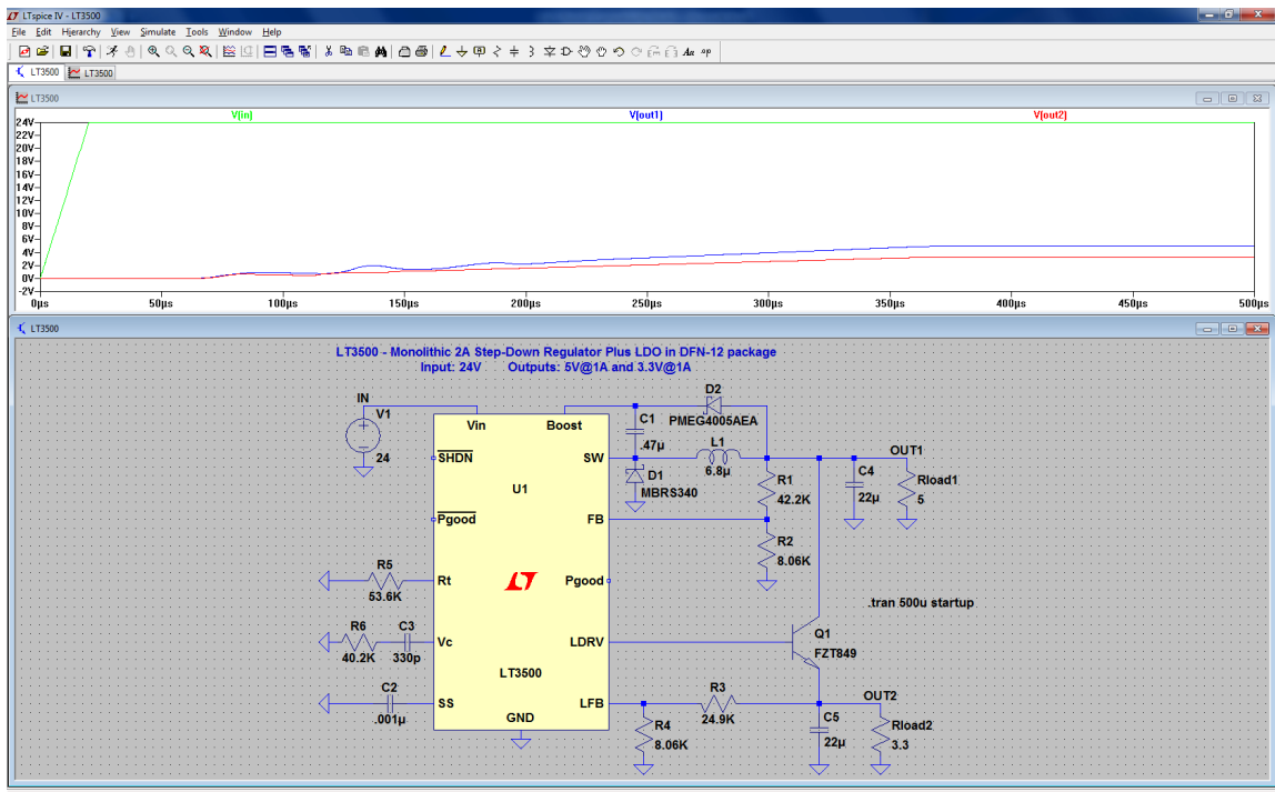
Figure 14 - LT3500 2A Buck Regulator LT Spice Simulation.
