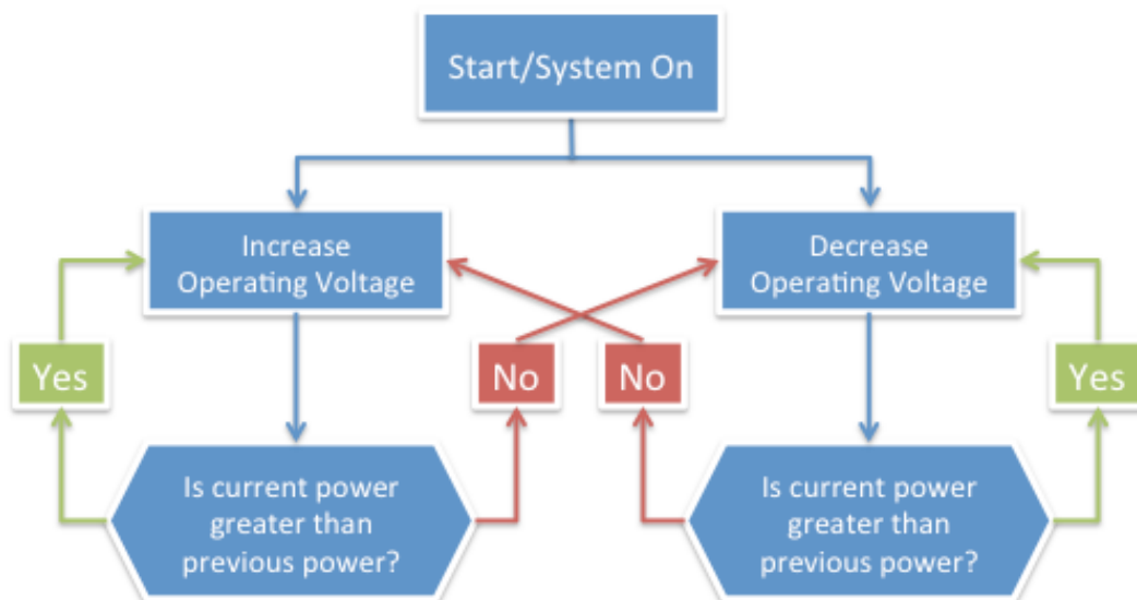
Figure 44 - Block Diagram of Perturb and Observe Method.
