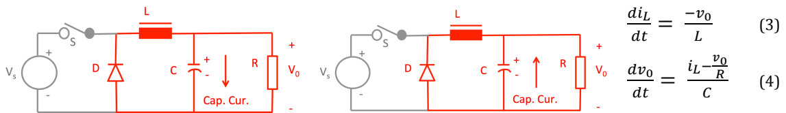
Figure 8 - Buck Converter Circuit OFF-State. Permission Pending.
