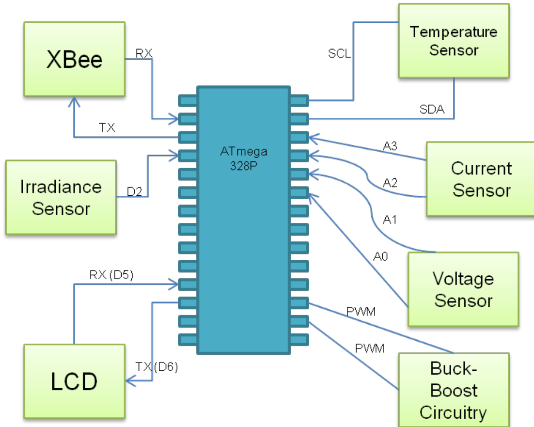
Figure 49 - PMCC Microcontroller Interfacing with Peripherals. [25]
