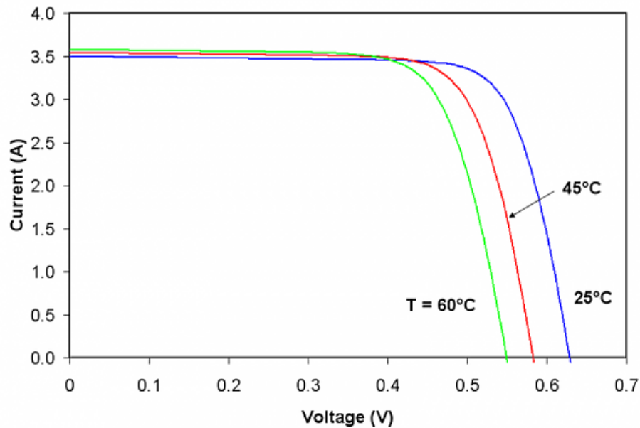
Figure 5 - Temperature effect on PV cell performance. Permission requested from solarpower2day.net.
