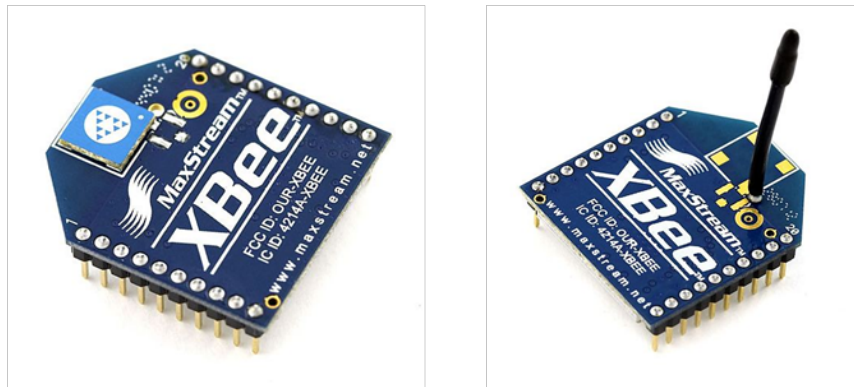
Figure 18 - XBee modules with two antenna types. Reproduced with permission from Sparkfun Electronics.
