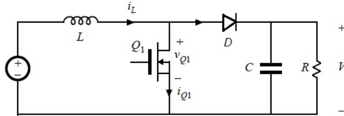
Figure 9 - Boost Converter Circuit.
