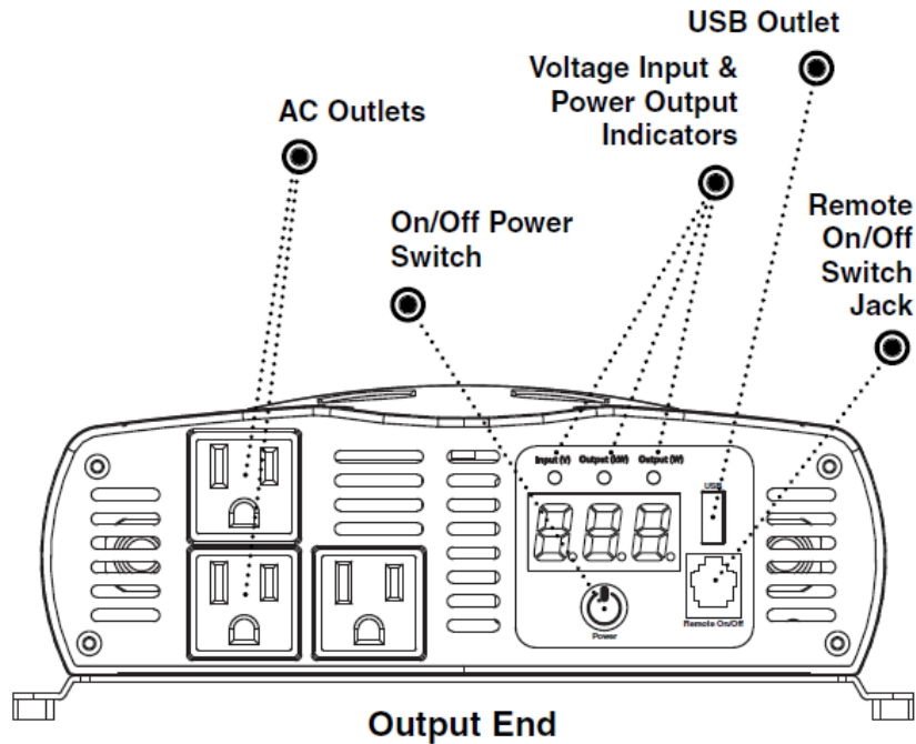
Figure 53 - Scobra CPI 1500 Power Inverter. Permission requested from Scobra.
