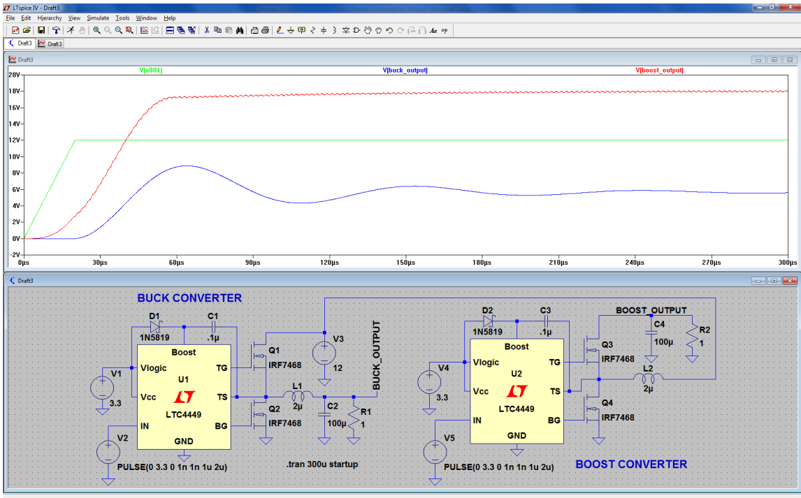
Figure 13 - Buck Converter and Boost Converter LT Spice Simulation.
