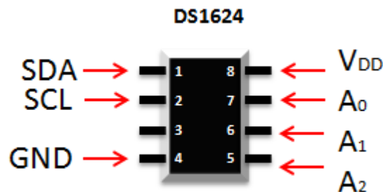
Figure 24 - DS1624 Digital Thermometer Pinout. [41]
