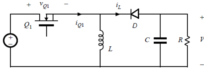
Figure 10 - Inverting Buck-Boost Converter Circuit.
