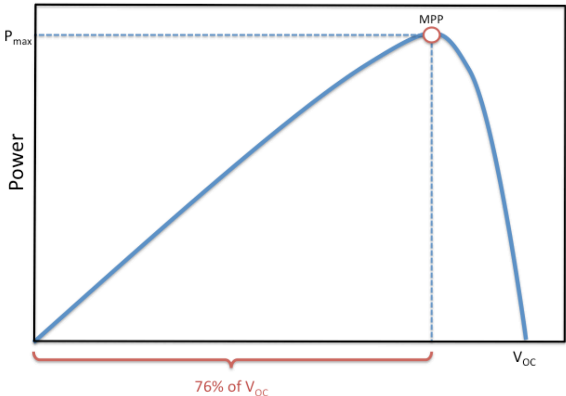
Figure 17 - The Constant Voltage Method for MPPT.
