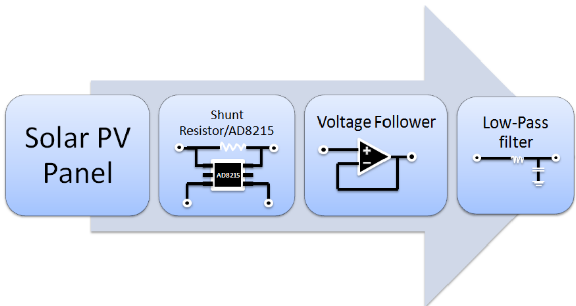
Figure 39 - Current Sensor Flow Chart.
