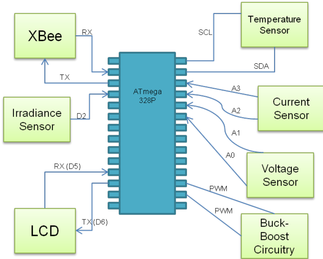
Figure 35 - PMCC Microcontroller Interfacing with Peripherals.
