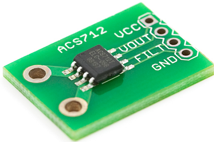
Figure 25 - ACS712 Current Sensor. Reproduced with permission from Sparkfun Electronics.
