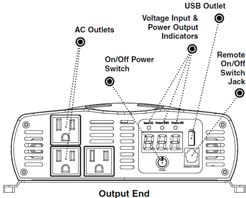
Figure 31 - Scobra CPI 1575 1500 Watt Power Inverter. Permission requested from Scobra.
