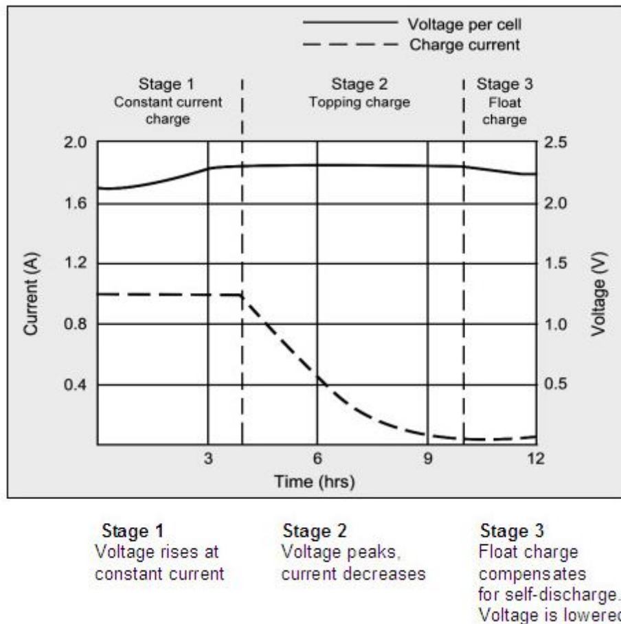
Figure 28 - Charging diagram for a typical lead-acid battery. Permission requested from Battery University.
