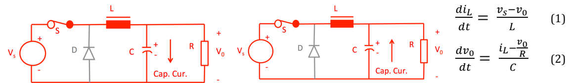
Figure 7 - Buck Converter Circuit ON-State. Permission Pending.
