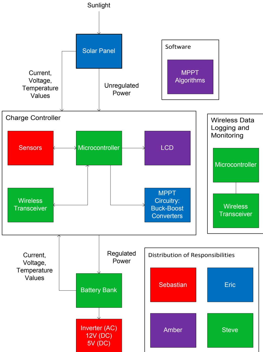
Figure 48 - Overall System Block Diagram with Group Member Responsibilities.
