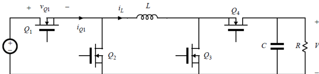
Figure 11 - Non-Inverting Buck-Boost Converter Circuit.
