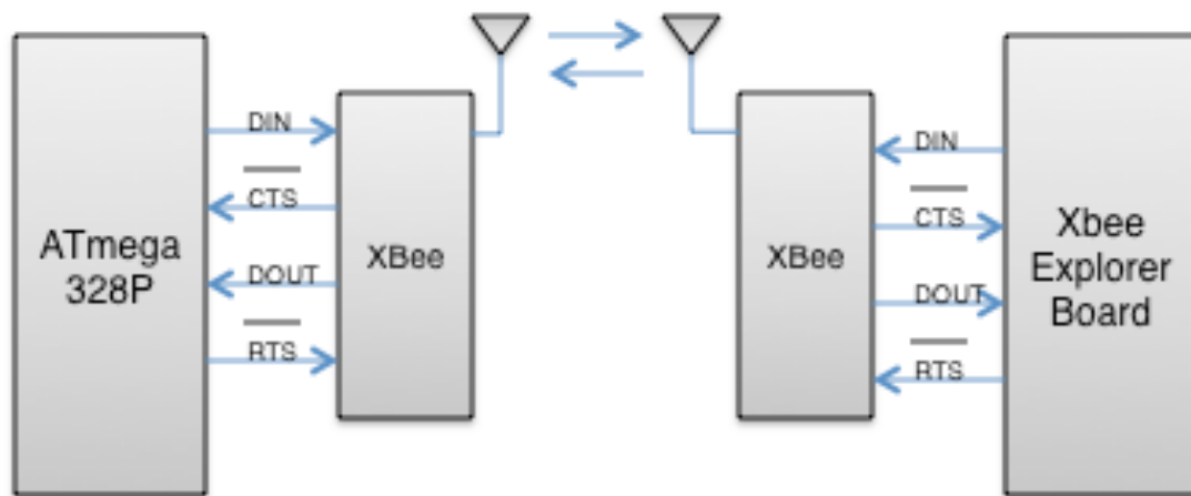
Figure 42 - Xbee to microcontroller configuration. [35]
