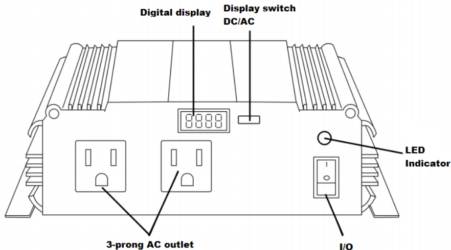
Figure 30 - Power Bright PW 1500 Inverter. Permission requested from Power Bright.
