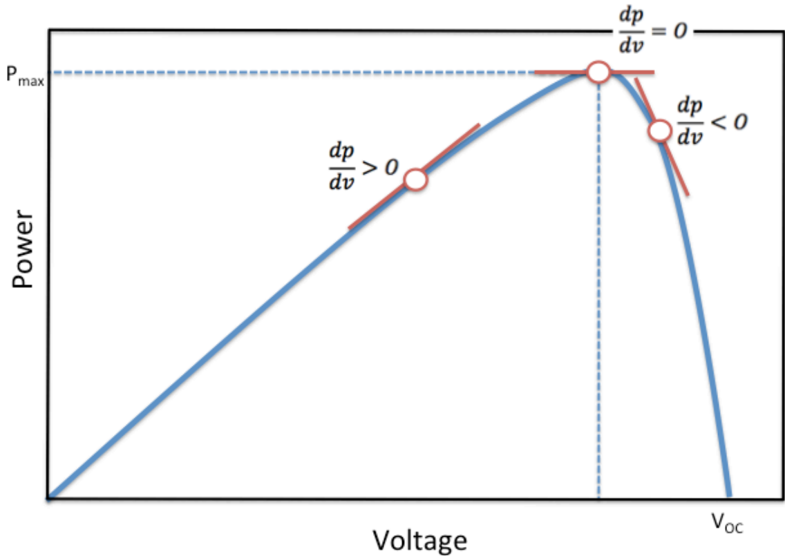
Figure 16 - The Incremental Conductance Method for MPPT.
