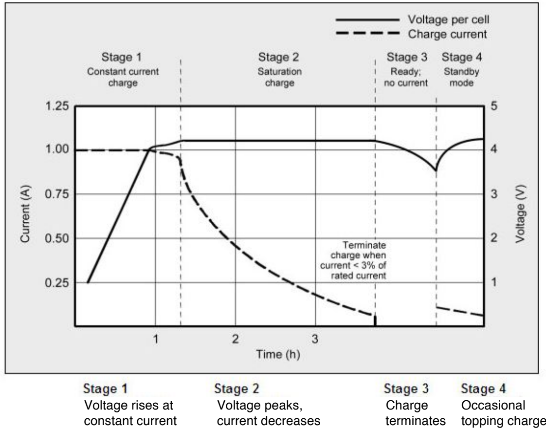
Figure 29 - Lithium-Ion Charging Diagram. Permission Requested from Battery University.
