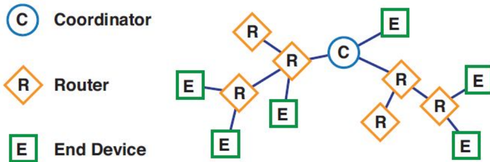
Figure 19 - ZigBee Mesh Network. Permission requested from Digi.
