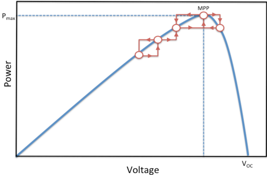
Figure 15 - The Perturb and Observe Method for MPPT.
