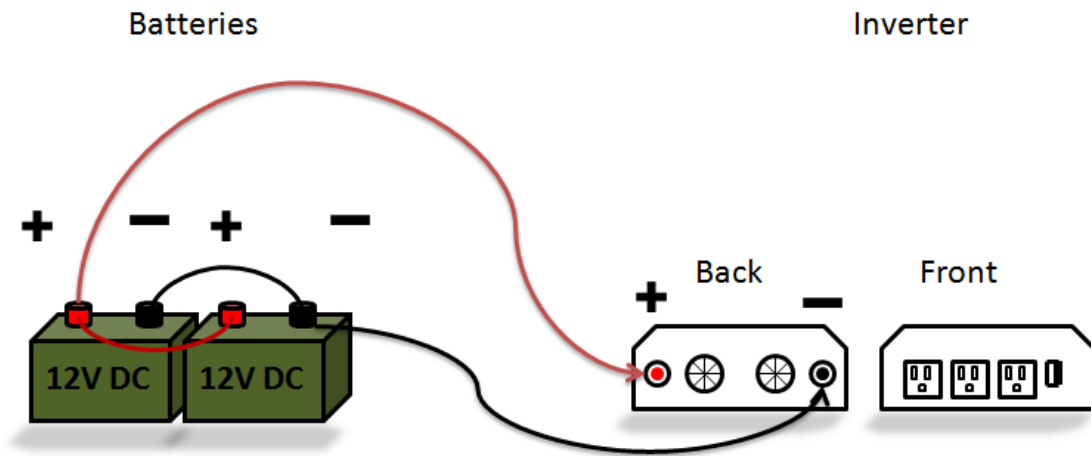
Figure 54 - Battery Bank to Inverter Connection.
