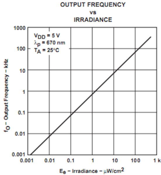
Figure 27 - Output Frequency vs. Irradiance Graph. Permission requested from Texas Instruments.
