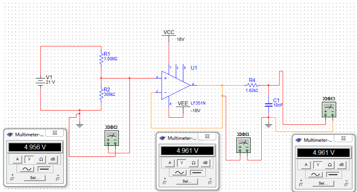
Figure 38 - Voltage Sensor Circuit.
