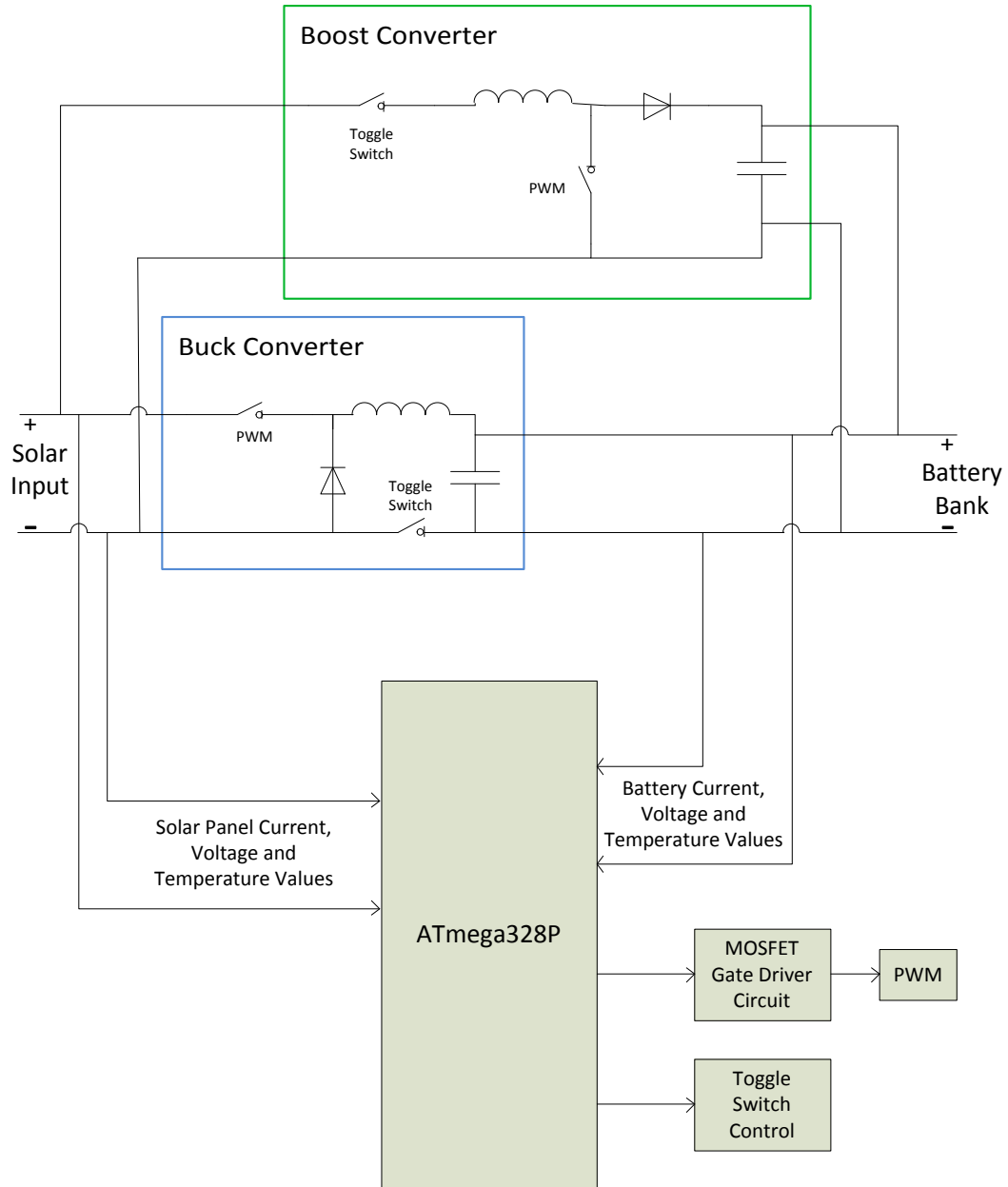
Figure 45 - Buck-Boost Circuit Diagram for MPPT.
