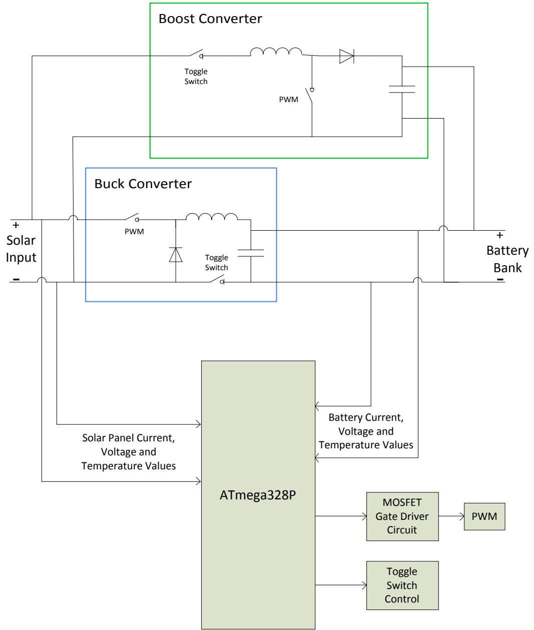
Figure 52 - Buck-Boost Circuit Design for MPPT.
