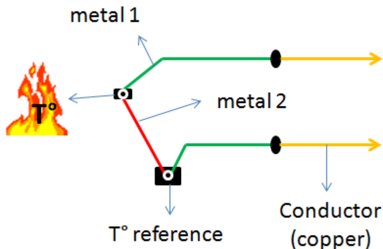
Figure 21 - Thermocouple schematic. [38]
