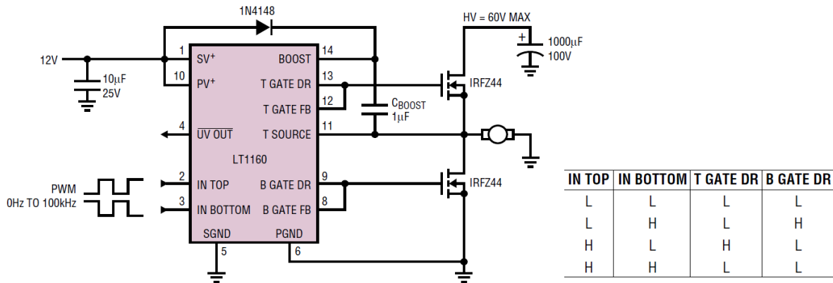
Figure 12 - LT1160 Half-Bridge Driver. Permission requested from Linear Technologies.
