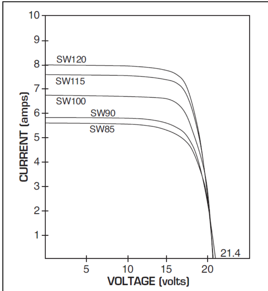
Figure 55 - SunWize SW-Series IV Characteristics. [61]
